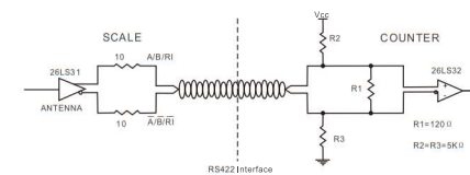
RS422 Interface
